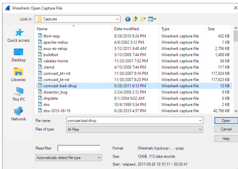
Figure 36. “Open” on Microsoft Windows
